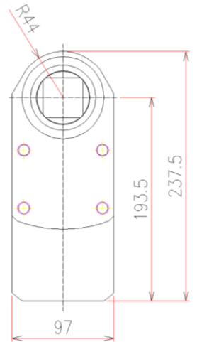
Mounting plate drawing
